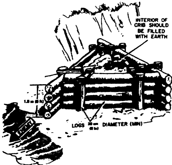
Figure 3-10. Triangular log crib used as a roadblock.
